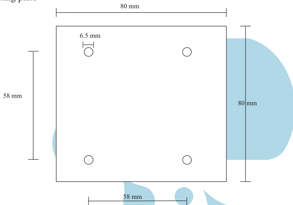
Rearview of mounting plate
